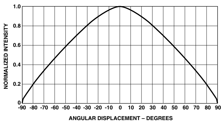
Figure 7. Radiation Pattern.
