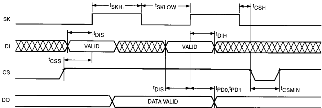
Figure 1. Synchronous Data Timing (8)
