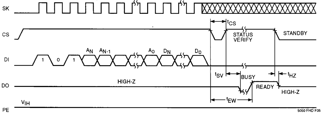
Figure 3. Write Instruction Timing (8)
