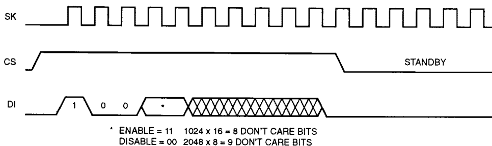
Figure 5. EWEN/EWDS Instruction Timing (8) (9)
