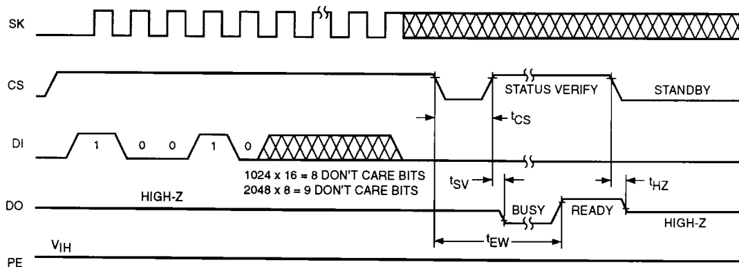
Figure 6. ERAL Instruction Timing (8)
