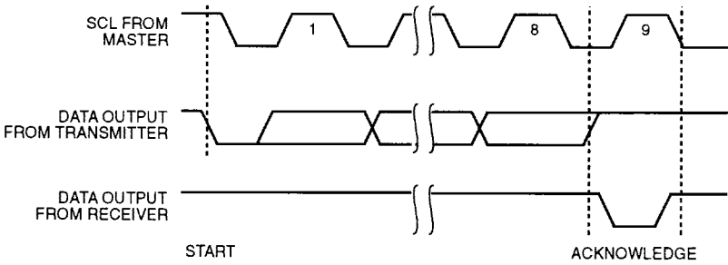
Figure 4. Acknowledge Timing
