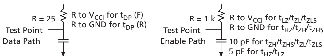
Figure 2-121 • AC Loading
