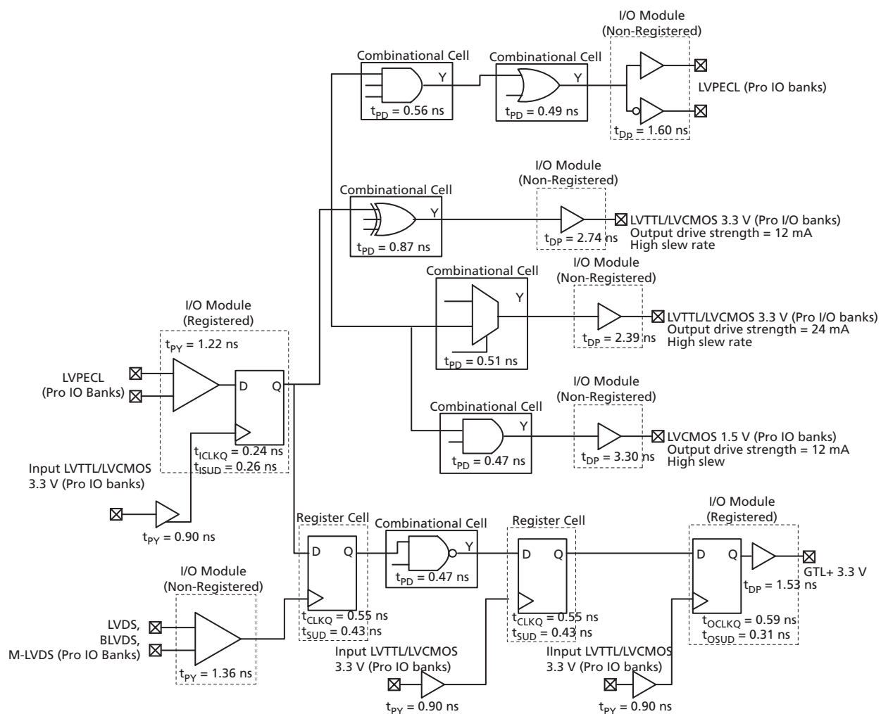
Figure 2-113 • Timing Model
