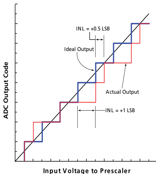
Figure 2-89 • Integral Non-Linearity (INL)
