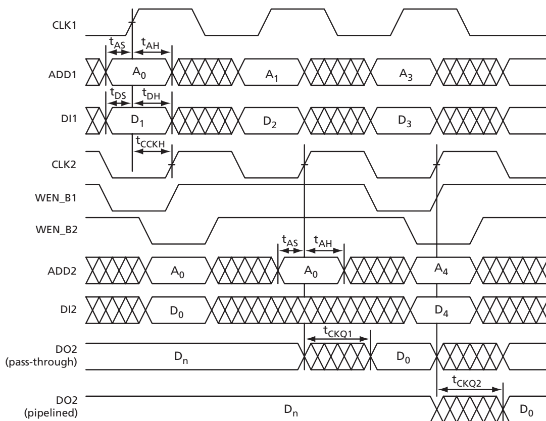
Figure 2-55 • Write Access After Write onto Same Address
