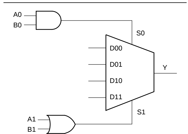
Figure 1 • C-module Implementation
