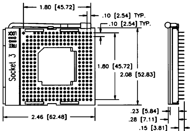
237 PIN PGA
