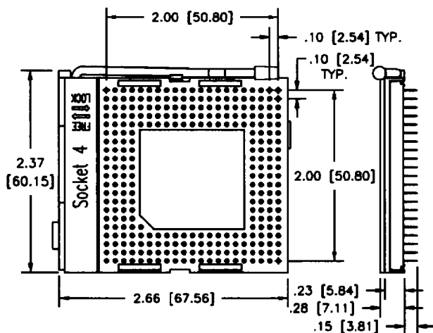
273 PIN PGA
