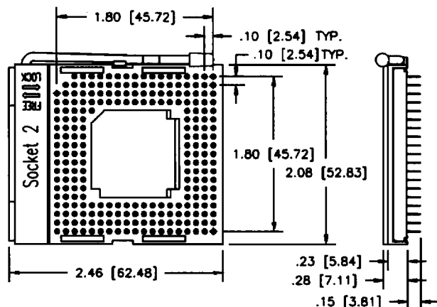
238 PIN PGA
