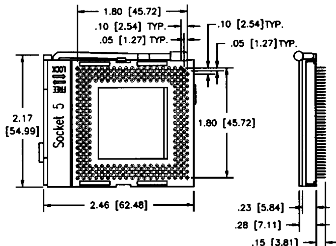
320 PIN IPGA
