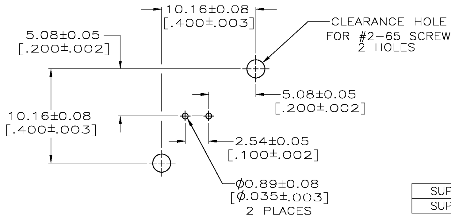
PCB CONFIGURATION
