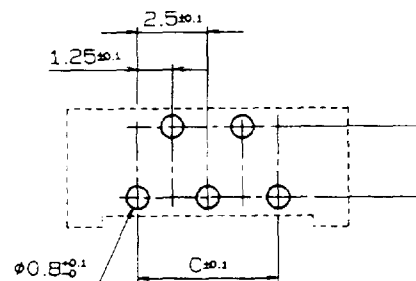
MOUNTING LAYOUT (t=1~1.6mm)
