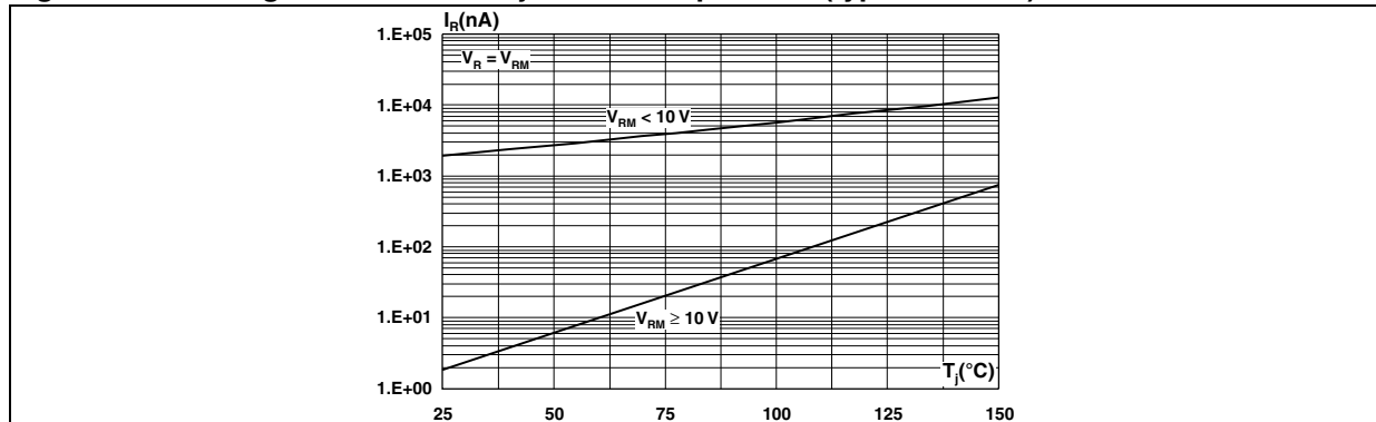
Figure 11. Leakage current versus junction temperature (typical values)
