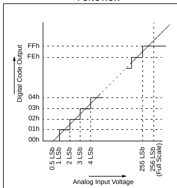
FIGURE 9-3: ADC TRANSFER FUNCTION
