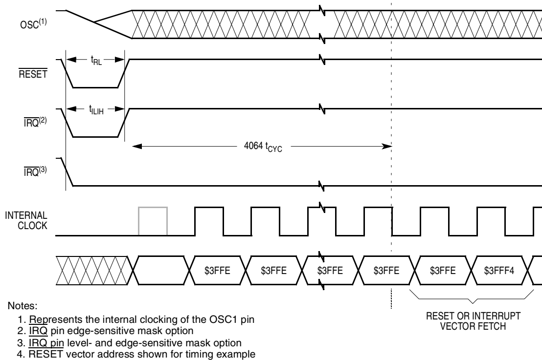
Figure 12-6. Stop Recovery Timing Diagram
