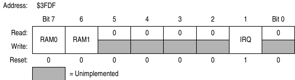
Figure 1-2. Option Register
