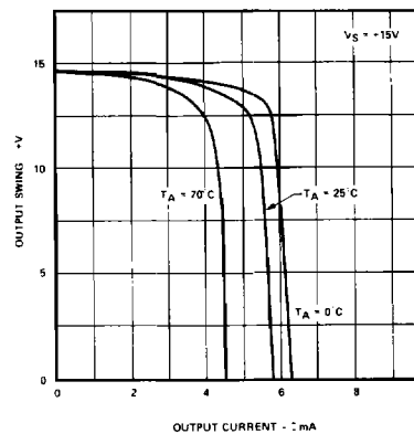
OUTPUT SWING
