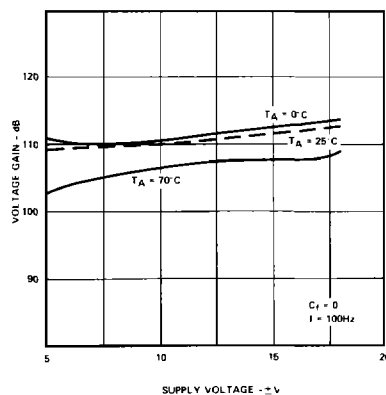
VOLTAGE GAIN
