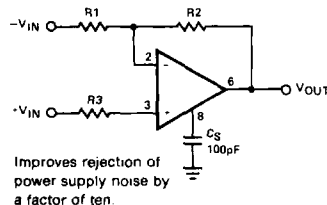
ALTERNATE FREQUENCY COMPENSATION
