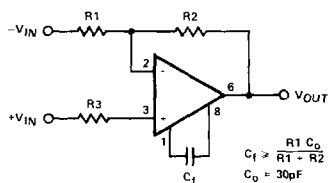
STANDARD COMPENSATION CIRCUIT
