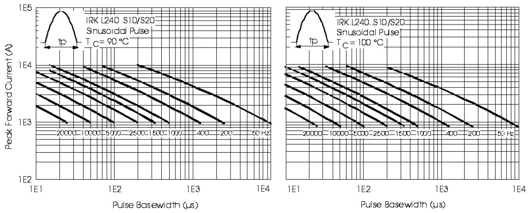
Fig. 22 - Frequency Characteristics
