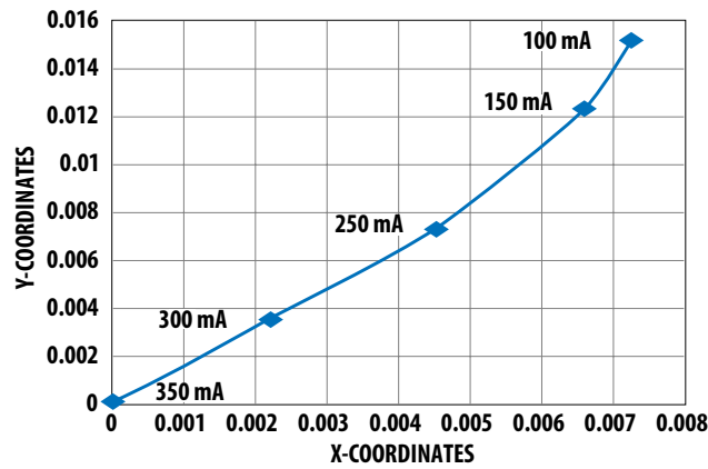
Figure 13. Chromaticity shift vs. current
