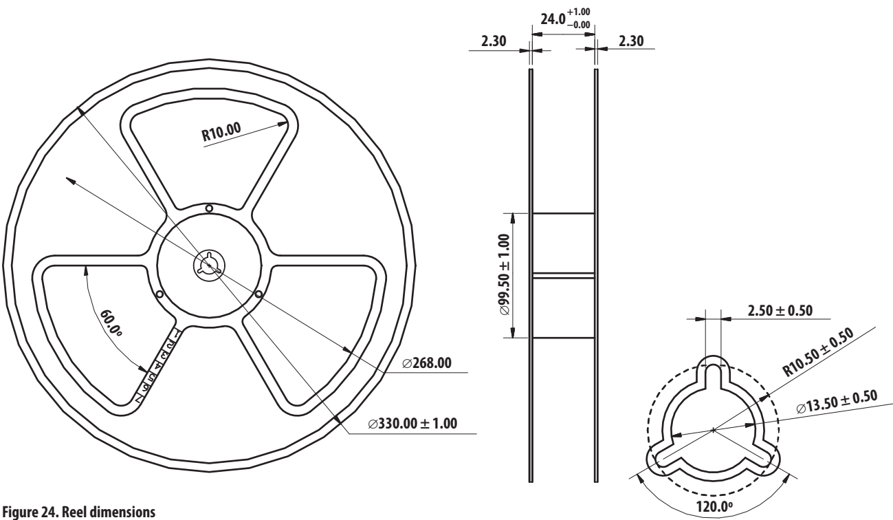
Figure 24. Reel dimensions
