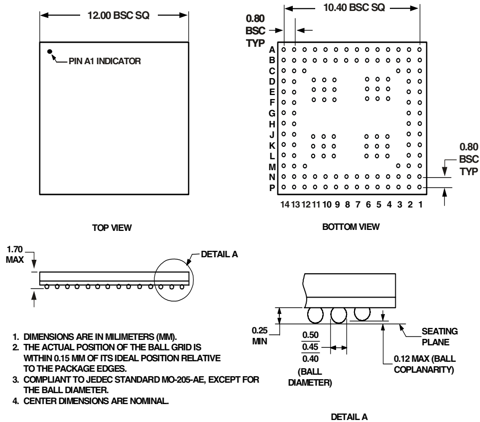
Figure 43. 136-Lead Chip Scale Package Ball Grid Array [CSP_BGA](BC-136-2)
