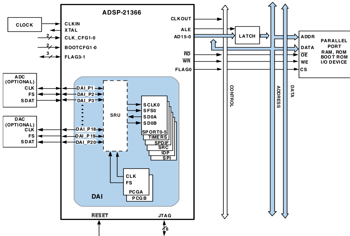
Figure 2. ADSP-21366 System Sample Configuration
