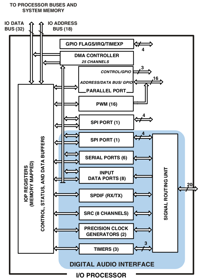
Figure 3. ADSP-21366 I/O Processor and Peripherals Block Diagram
