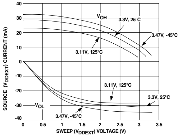
Figure 36. ADSP-21366 Typical Drive
