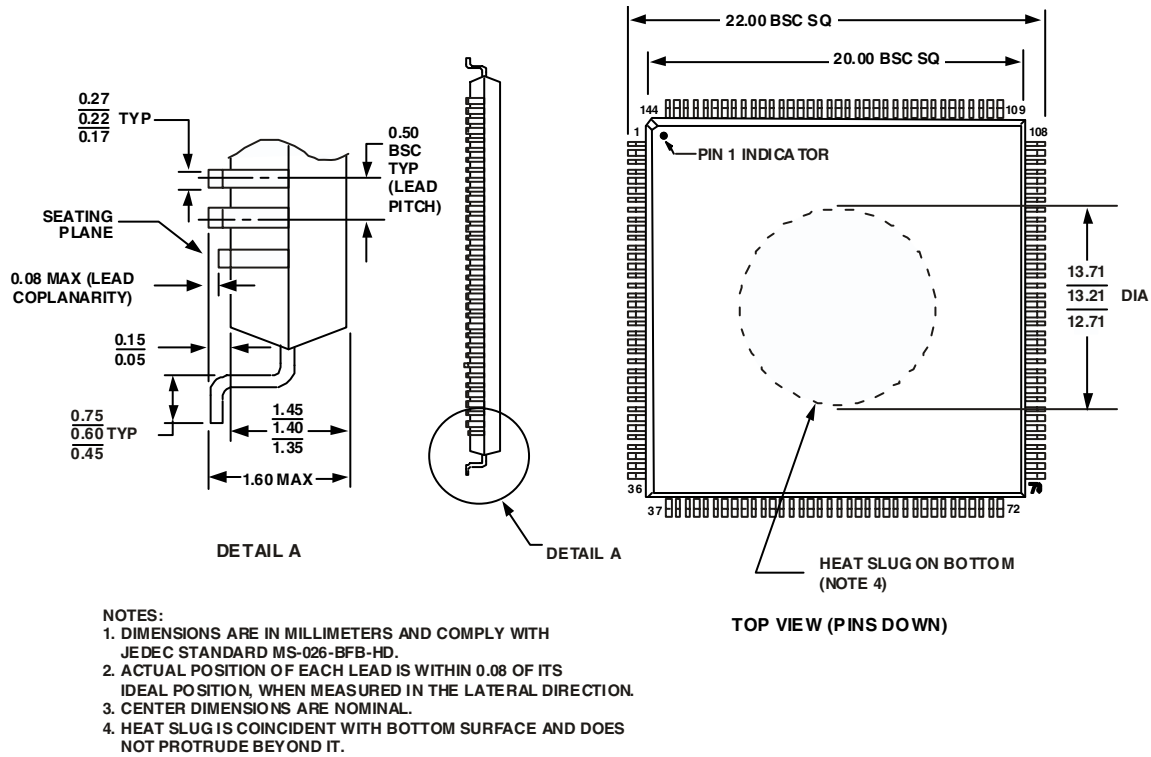
Figure 44. 144-Lead Low Profile Quad Flat Package, with Integrated Heatsink [LQFP_INT_HS] (SQ-144-3)
