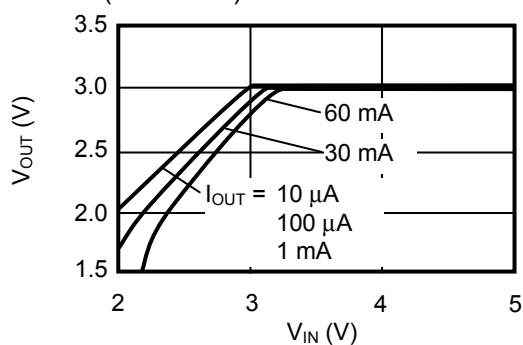
S-814A30A ( T_a = 25^\circ\text{C} )
