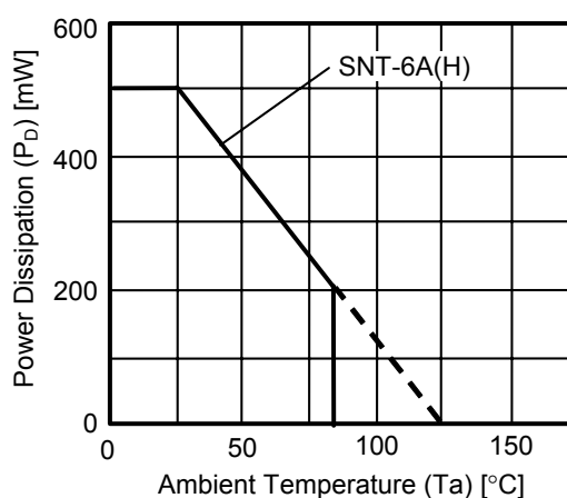
Figure 5 Power Dissipation of Package (Mounted on Printed Circuit Board)
