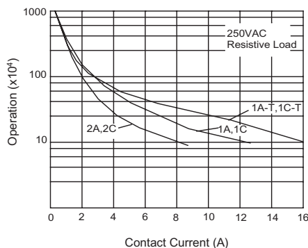
Life Curves
