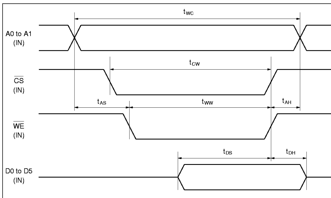
Figure 7 Register Write
