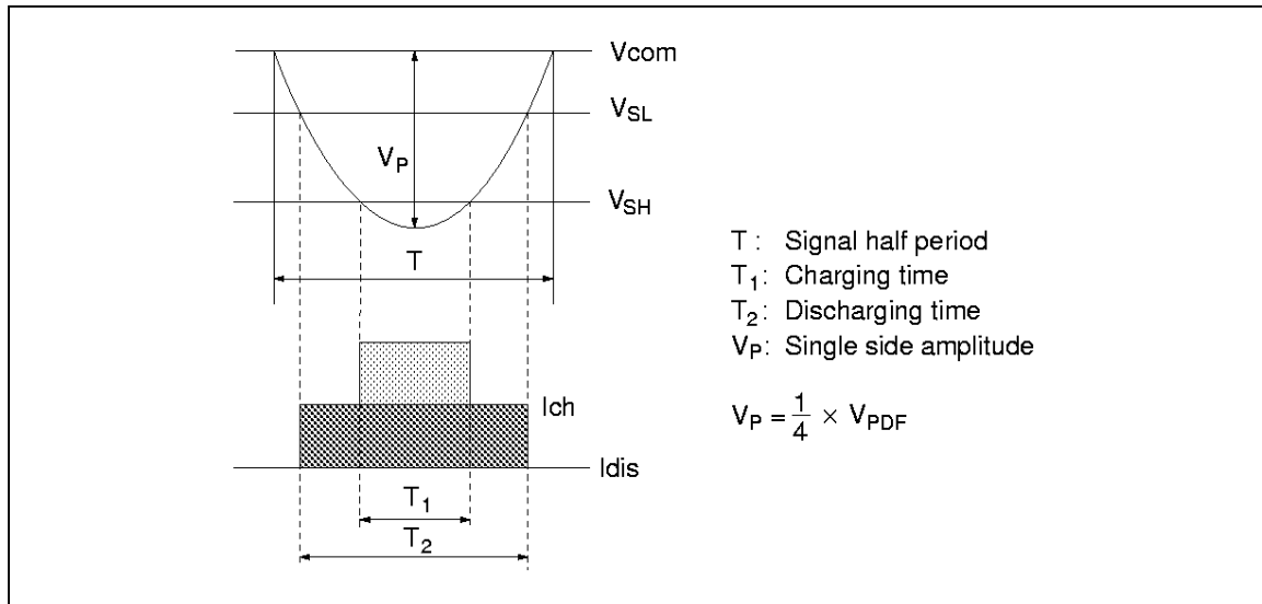
Figure 8-2 Amplitude Detection
