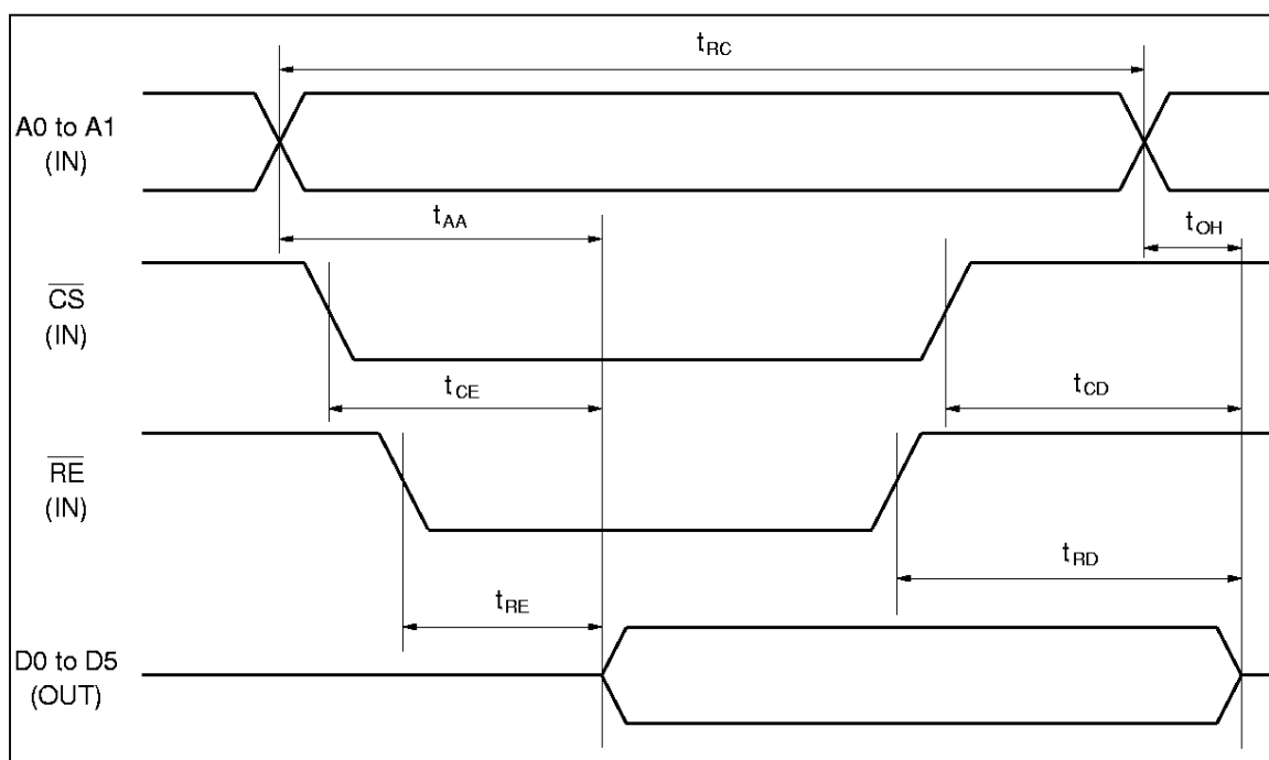
Figure 8 Register Read
