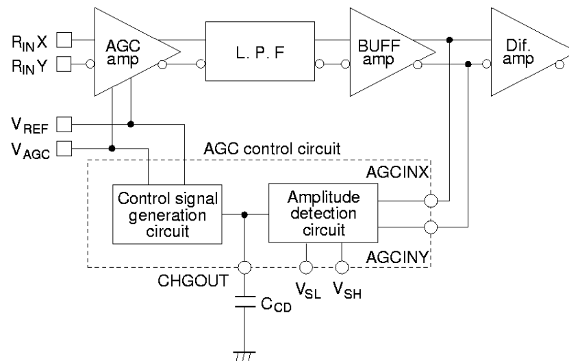
b. AGC Loop Structure, Example 2
