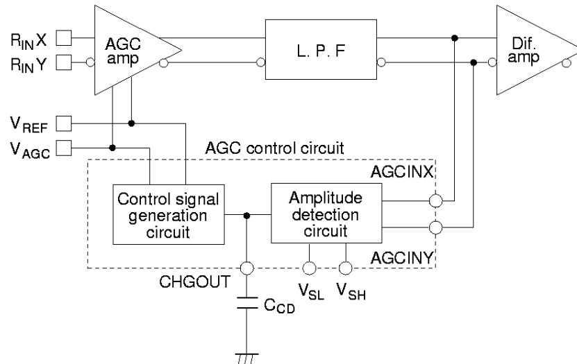
a. AGC Loop Structure, Example 1
