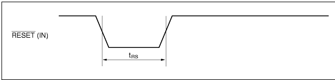
Figure 1 Reset Input
