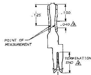
DETAIL Z SCALE 10:1
