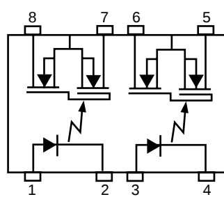
2 Form A/2 Form B, Dual 1 Form A/1 Form B
