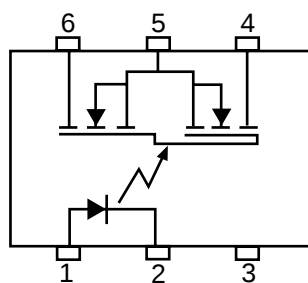
1 Form A/1 Form B
