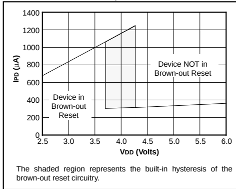
FIGURE 14-9: MAXIMUM I_{PD} vs. V_{DD} BROWN-OUT DETECT ENABLED (85°C TO -40°C, RC MODE)
