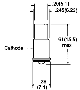
Available With Center Cathode MF200, F Series (90°)
