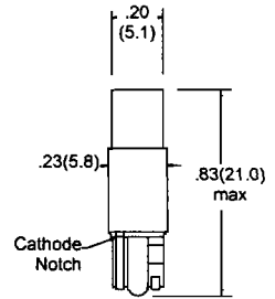
WB200, F Series (90°)
