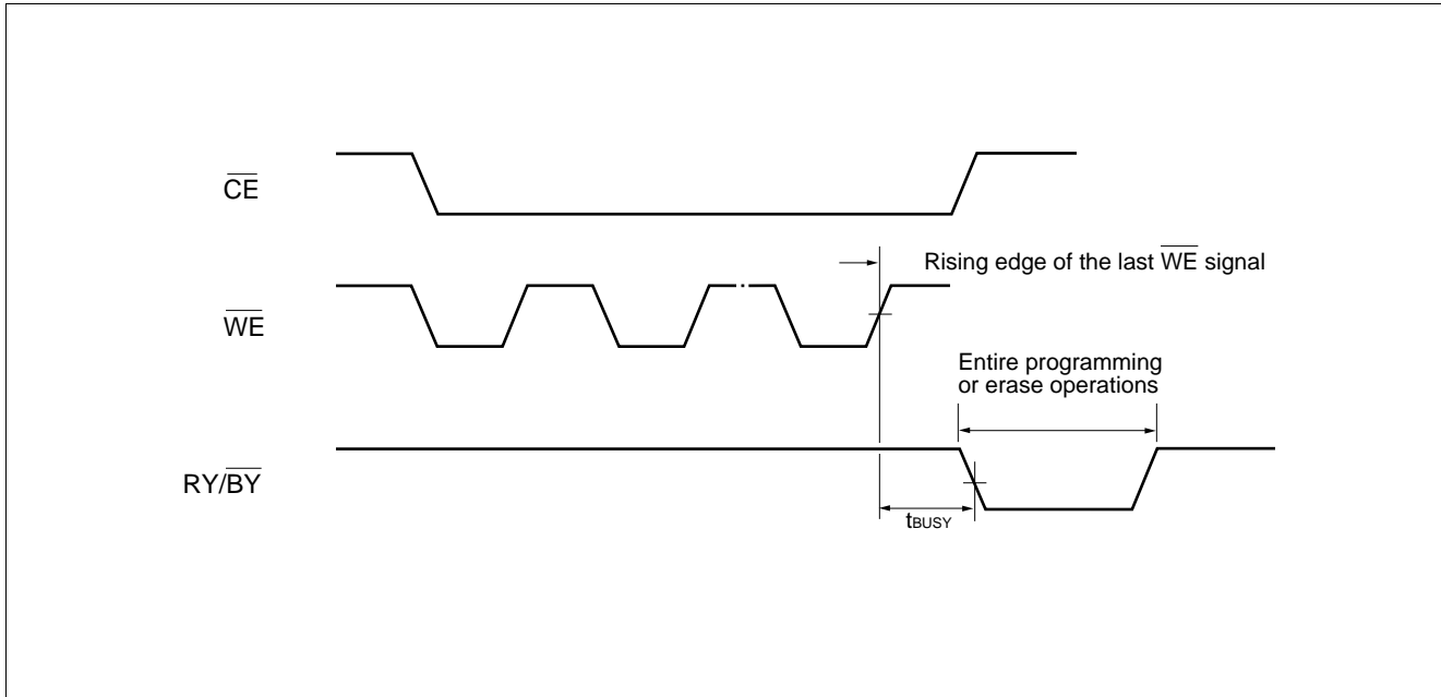
(8) RY/ \overline{\text{BY}} Timing Diagram during Program/Erase Operations
