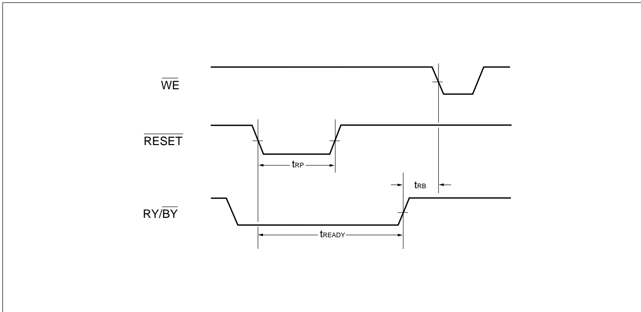
(9) \overline{\text{RESET}} /RY/ \overline{\text{BY}} Timing Diagram
