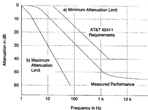
Figure 10. Typical Jitter Attenuation Curve
