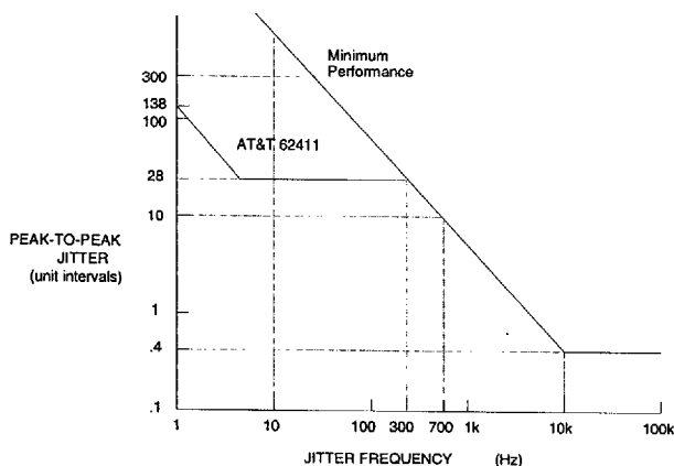
Figure 12. Minimum Input Jitter Tolerance of Receiver
