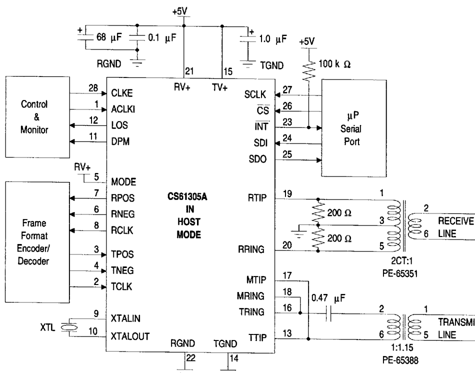
Figure A2. T1 Host Mode Configuration
