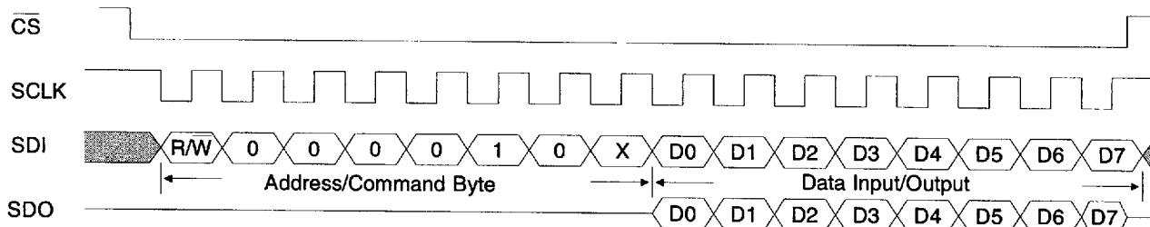
Figure 13. Input/Output Timing
