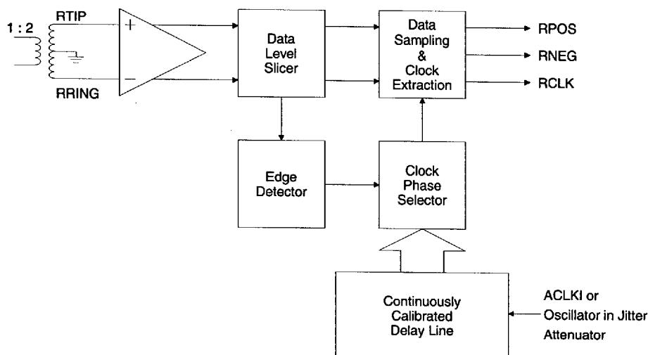
Figure 11. Receiver Block Diagram
