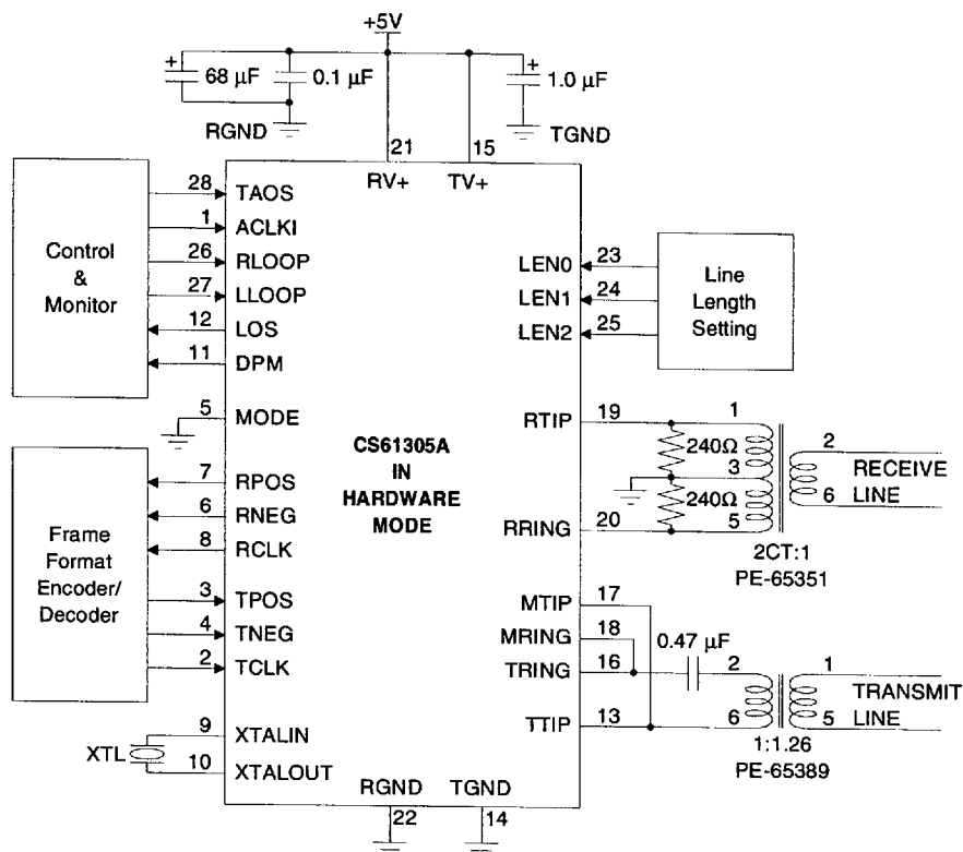
Figure A3. 120 Ω, E1 Hardware Mode Configuration
