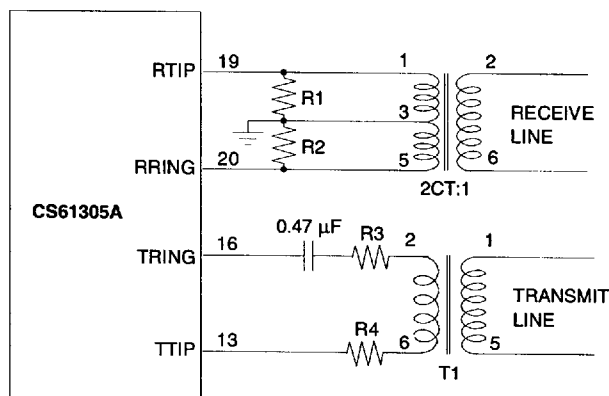
Figure A1. Line Interface Circuitry
