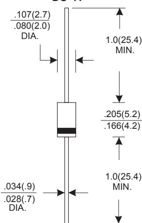
DO-41
