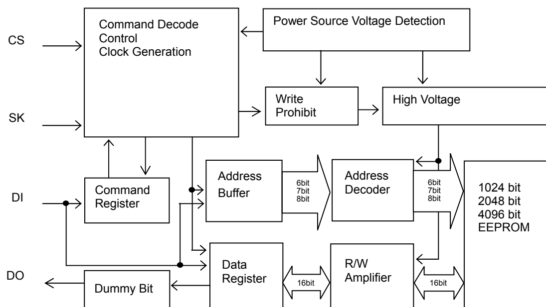
Figure 2: Block Diagram
