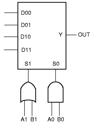
Figure 2 • C-Module Diagram
