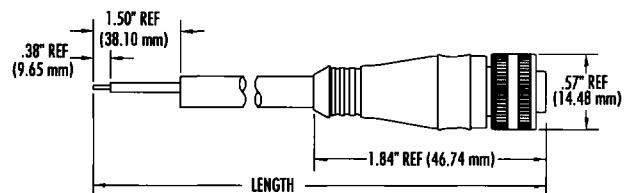
Straight Male Plug / 5 Pole
