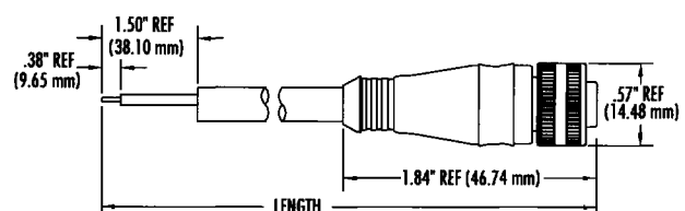
Straight Female Plug / 5 Pole
