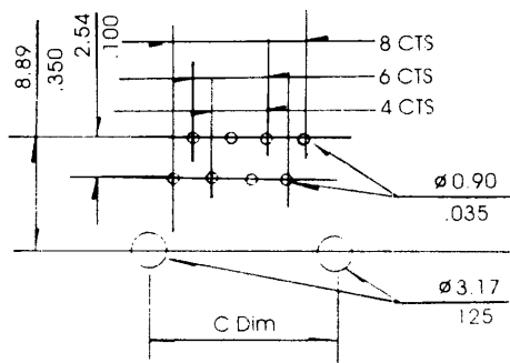
Mounting hole patterns for standard
