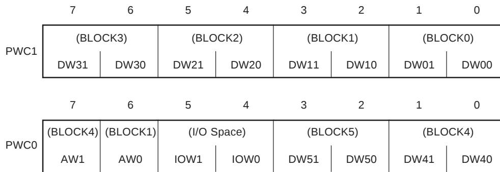
Figure 4-2. Memory Wait Control
