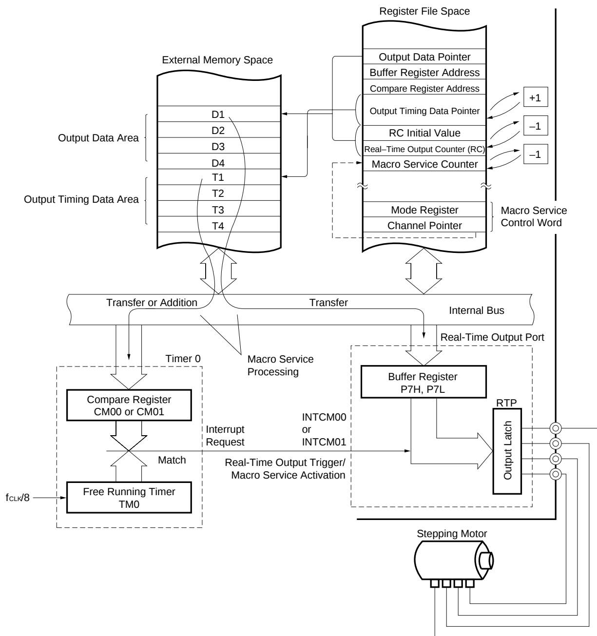
Figure 9-3. Real-Time Output Port Stepping Motor Control
