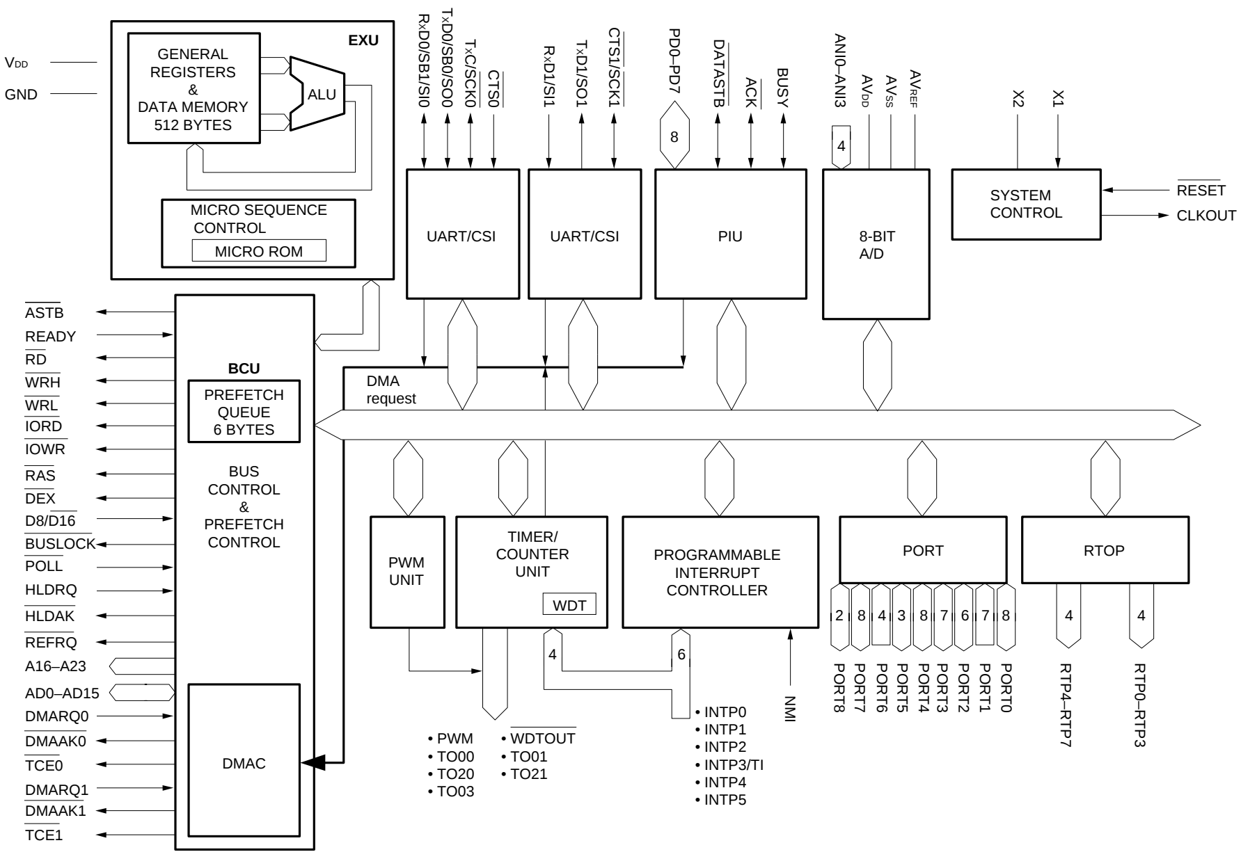
INTERNAL BLOCK DIAGRAM
