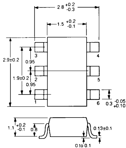
UPC2709T/UPC2712T PACKAGE OUTLINE T06
