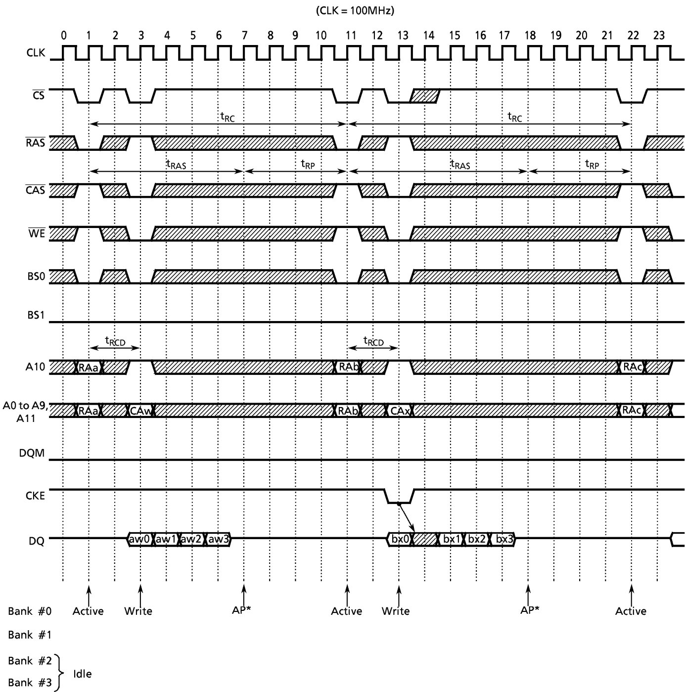
Figure 10. Auto Precharge Write (Burst Length=4)
