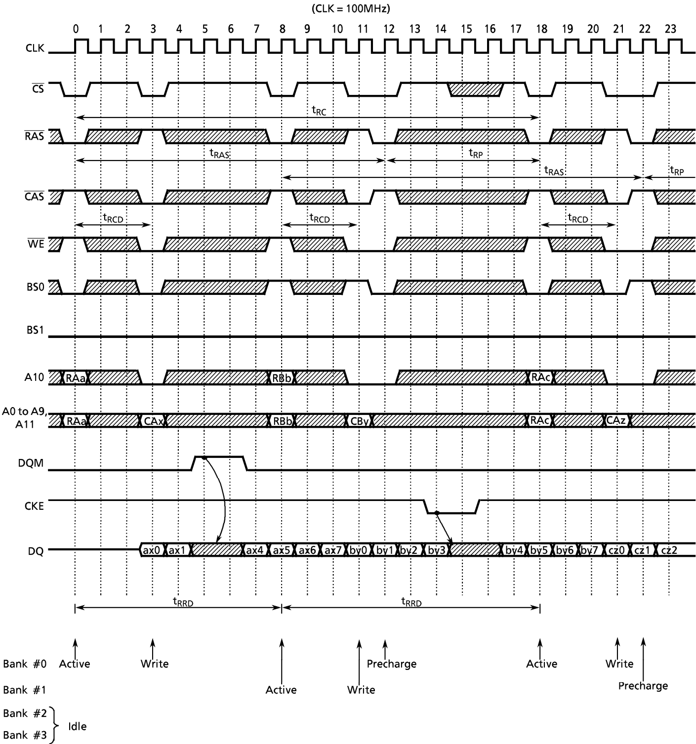
Figure 5. Interleaved Bank Write (Burst Length=8)
