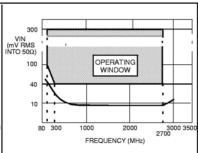
Fig. 5b Typical input sensitivity (Prescaler enabled, PE=1)
