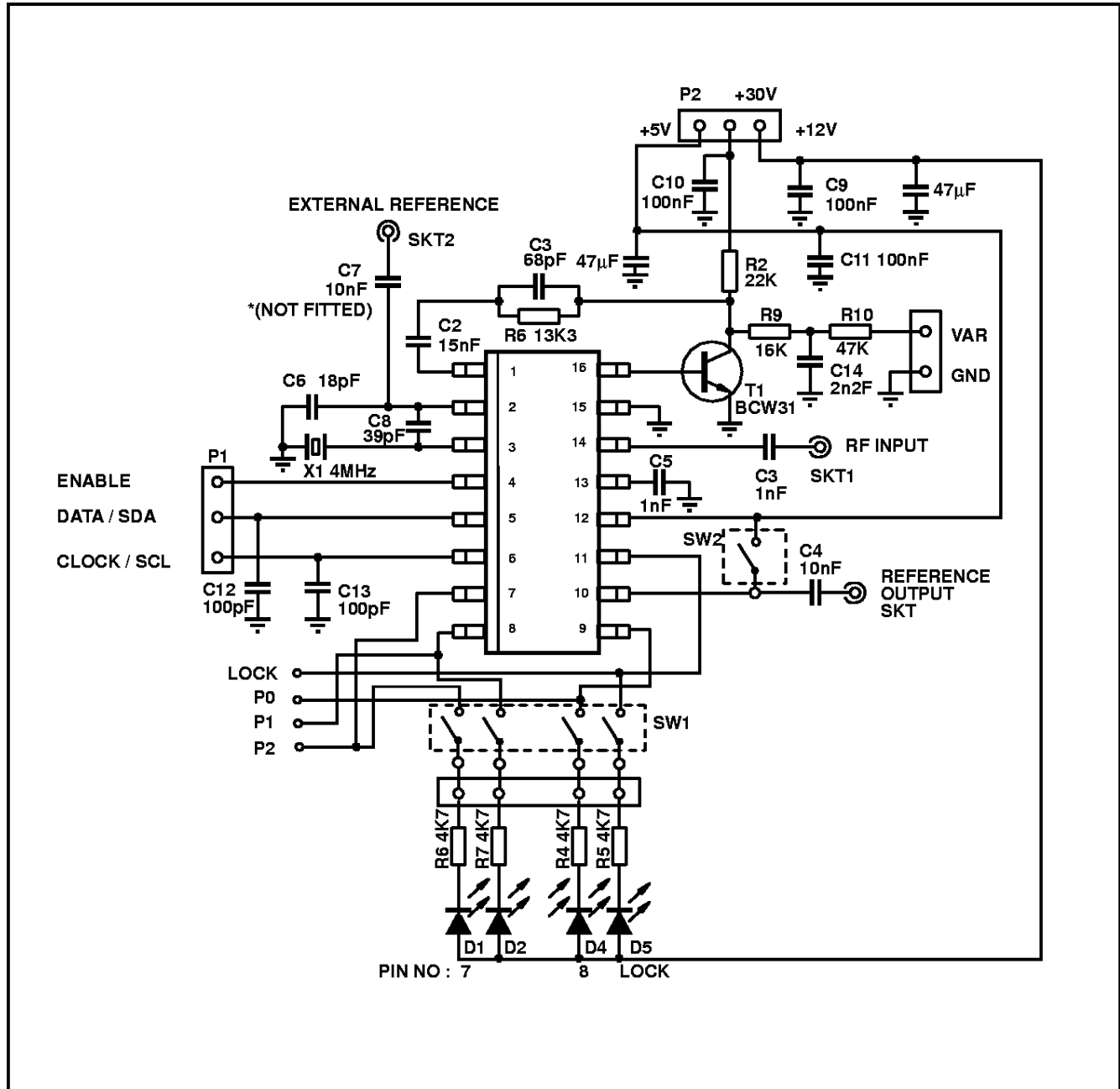
Fig. 8 Evaluation board
