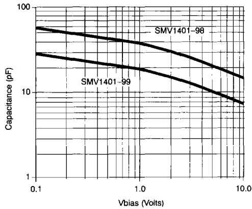
Capacitance vs. Voltage
