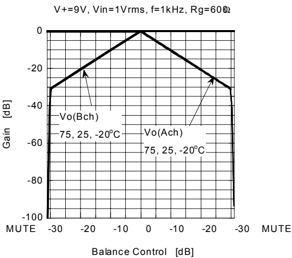
Gain vs Balance Control
