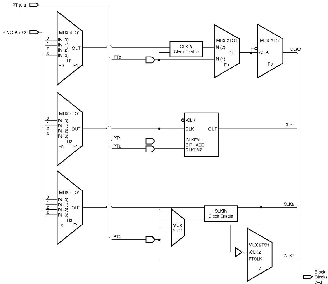
Figure 4. Clock Generator
