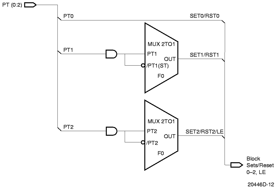
Figure 5. Set/Reset Generator
