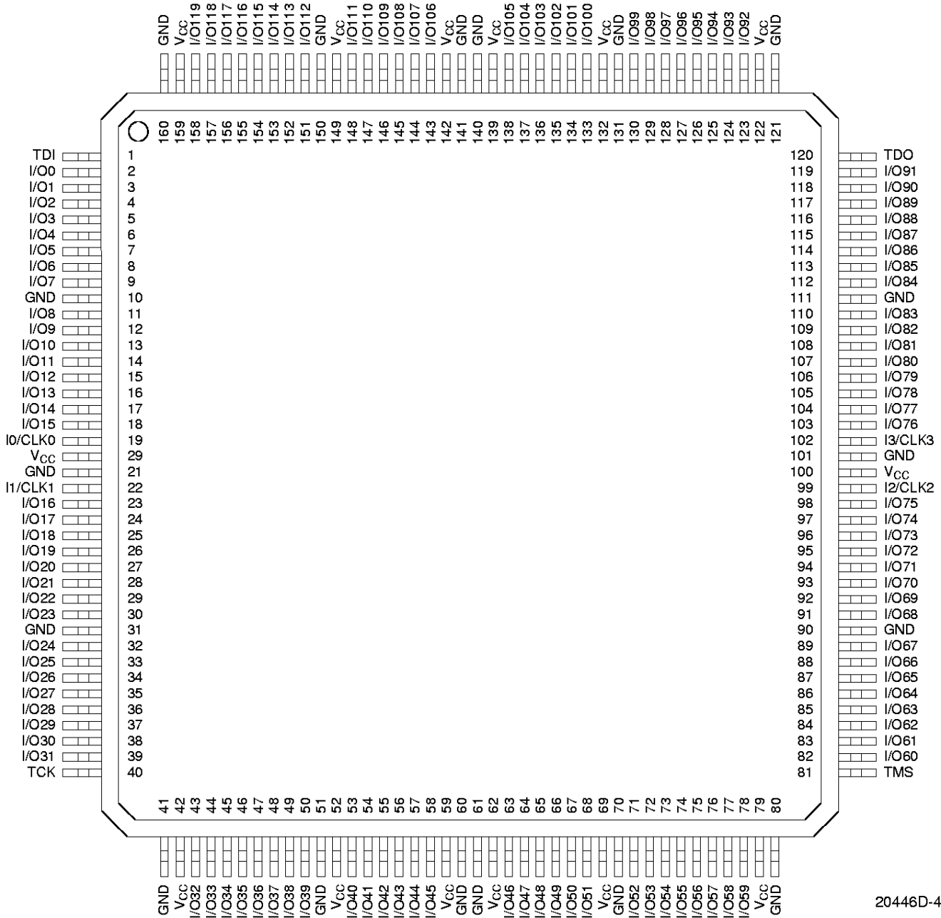
160-Pin PQFP
