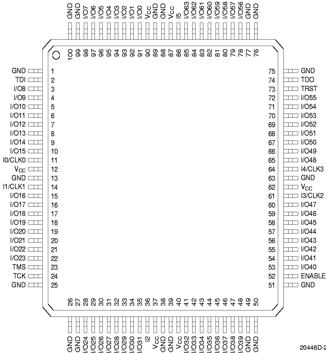
100-Pin TQFP
