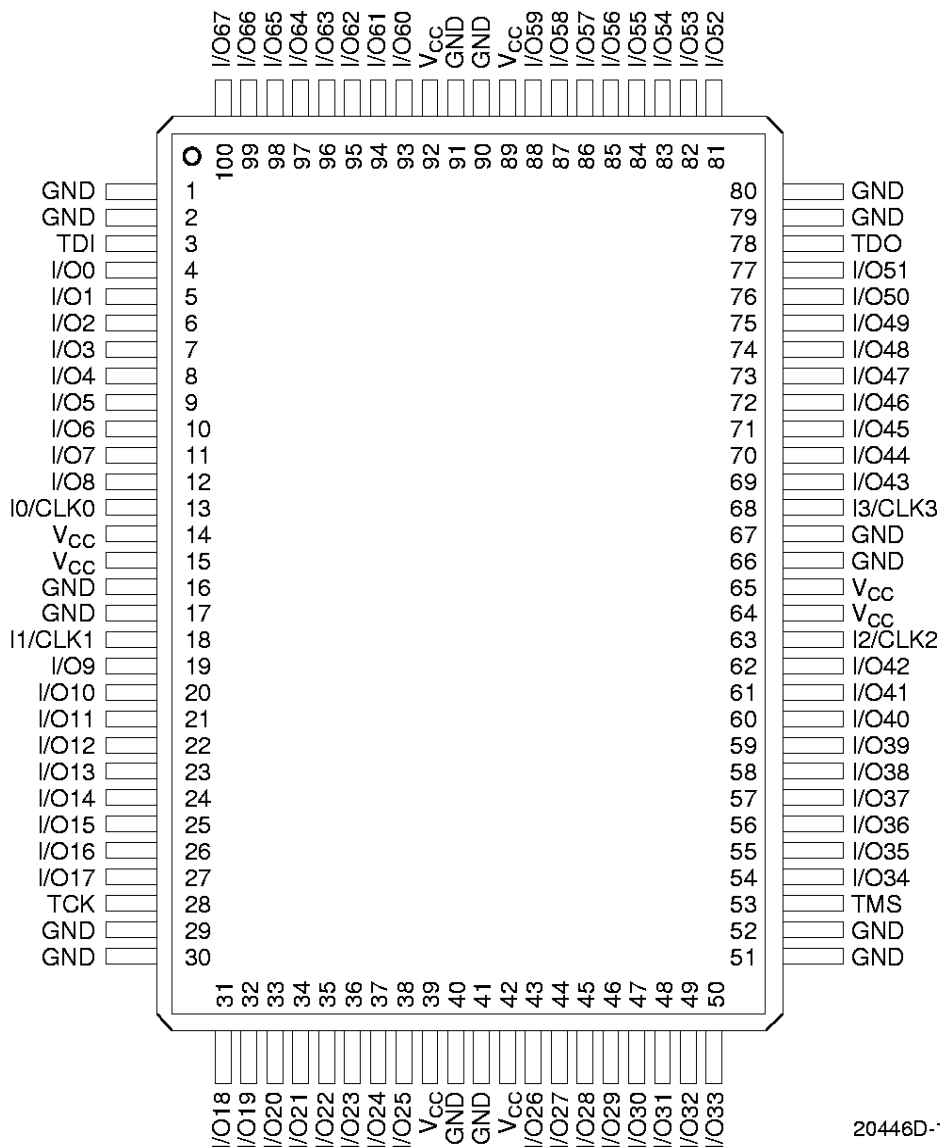
100-Pin PQFP
