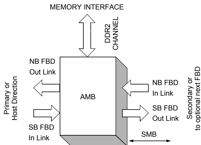
Figure 12 : Advanced Memory Buffer Interface Block Diagram
