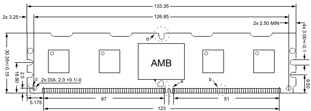
Figure 17 : FBDIMM Physical Dimension -1 (For PCB) : 128Mbx8 based 128Mx72 Module (1Rank) M395T2863DZ4
