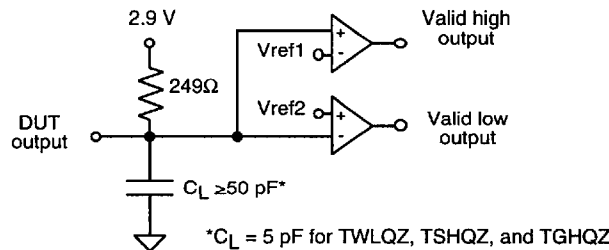
Tester Equivalent Load Circuit
