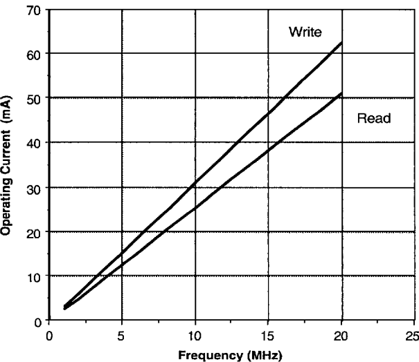
Operating Current vs. Frequency @ 225°C
