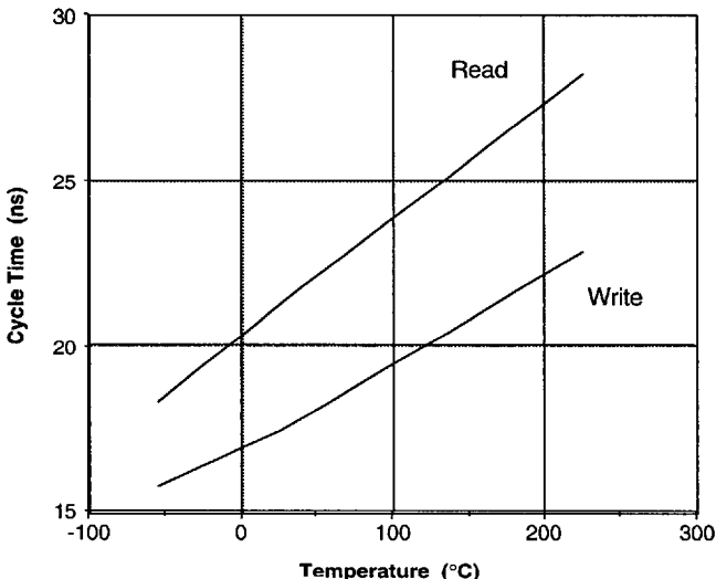
Cycle Times vs. Temperature
