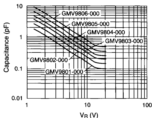
980X Series Capacitance vs. Voltage
