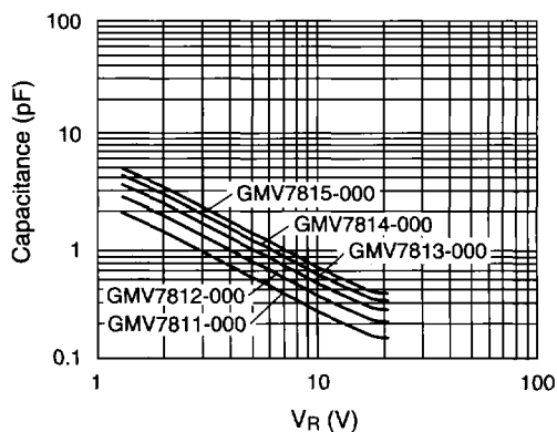
781X Series Capacitance vs. Voltage
