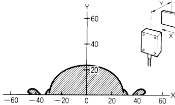
V600-HS63 + V600-D2KR16
