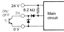
Output Circuit
