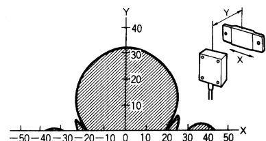
V600-HS63 + V600-D8KR12
