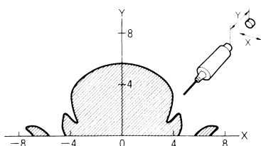
V600-HS51 + V600-D8KR12
