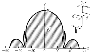
V600-HS63 + V600-D8KR04
