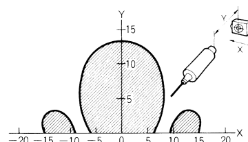
V600-HS51 + V600-D23P61
