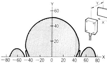
V600-HS63 + V600-D2KR16
