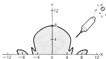
V600-HS51 + V600-D23P54
