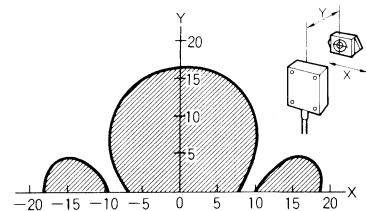
V600-HS61 + V600-D23P61
