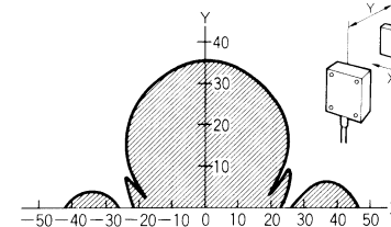
V600-HS63 + V600-D23P72
