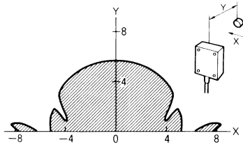
V600-HS61 + V600-D23P72
