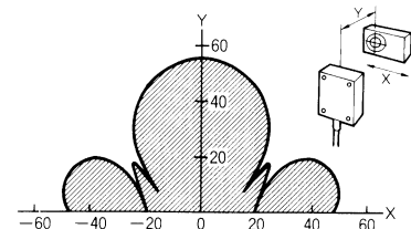
V600-HS63 + V600-D8KR12
