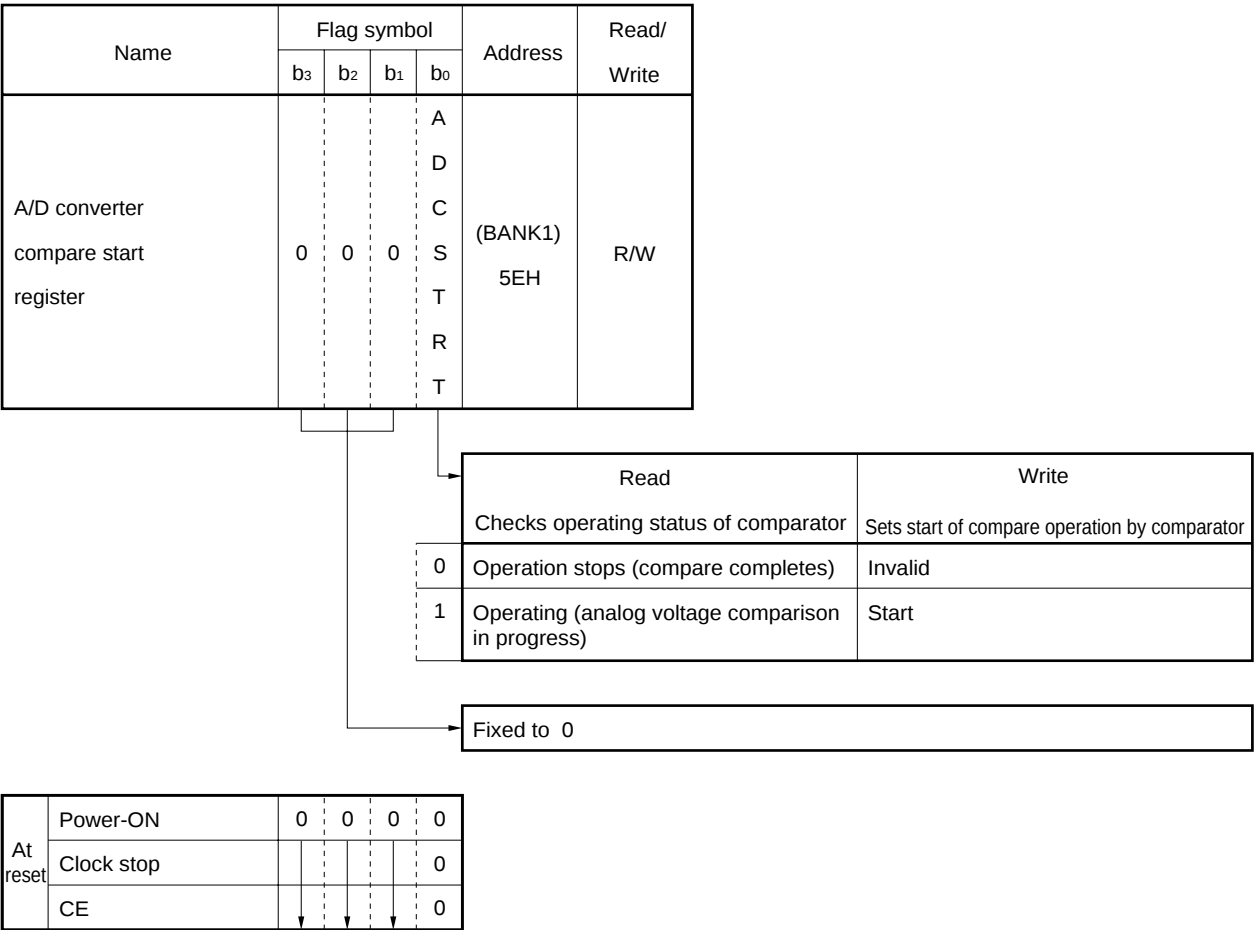
Figure 13-6. Configuration of A/D Converter Compare Start Register
