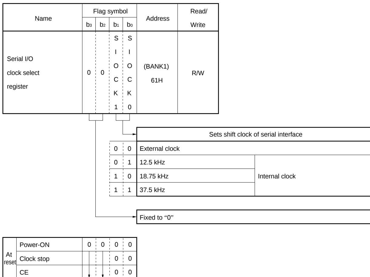
Figure 14-2. Configuration of Serial I/O Clock Select Register
