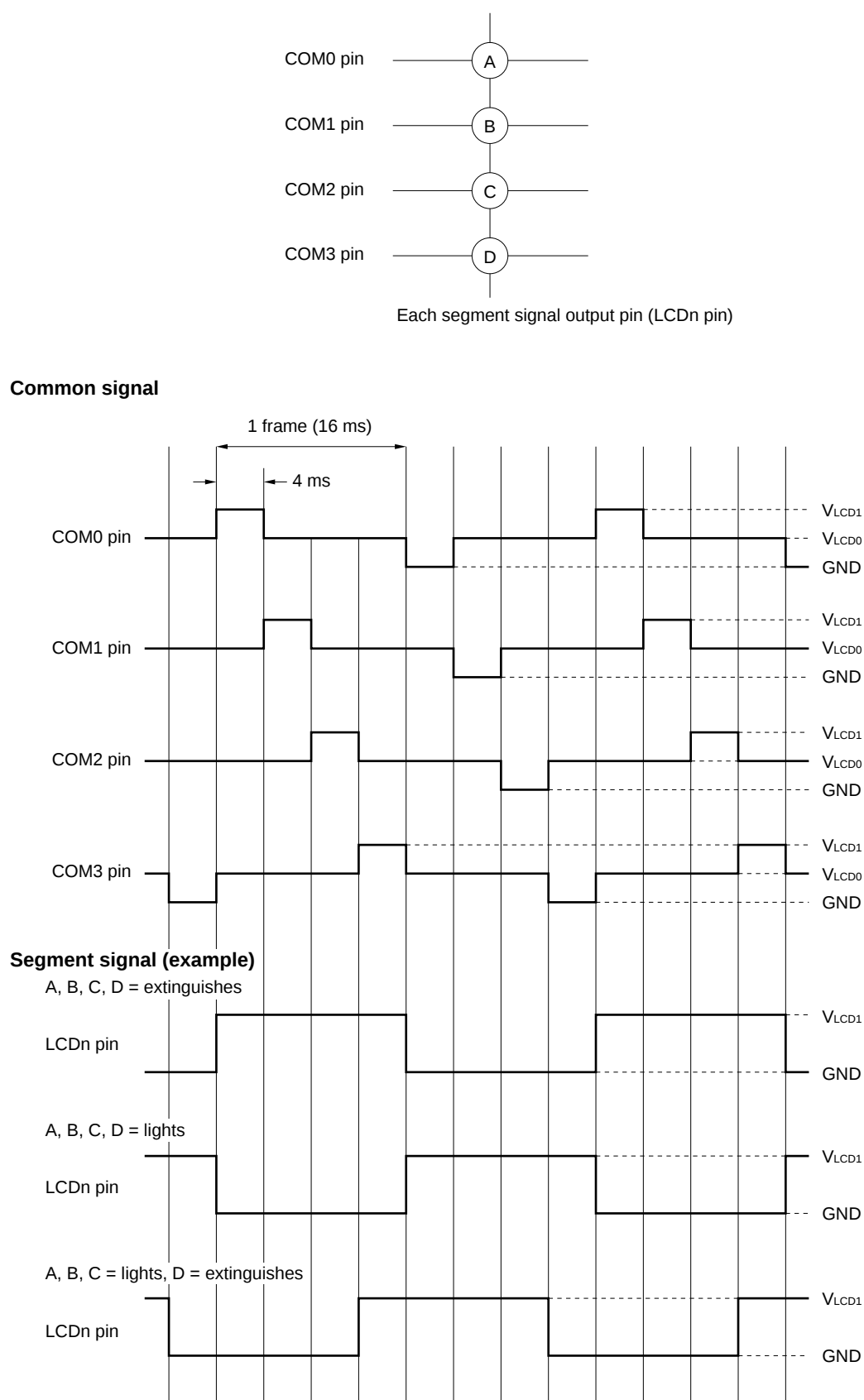
Figure 18-7. Common Signal and Segment Signal Output Waves
