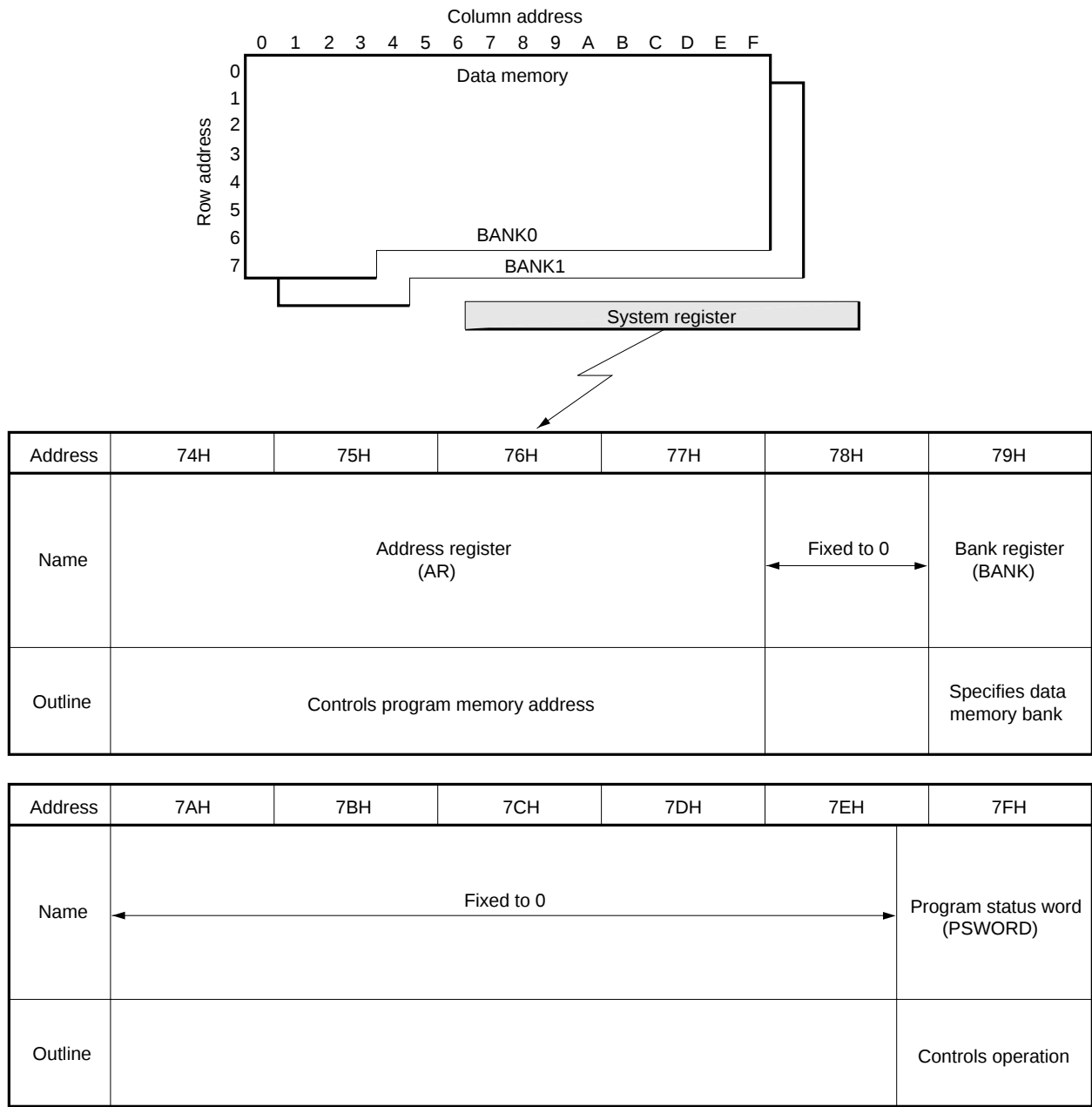
Figure 5-1. Location of System Register on Data Memory and Outline
