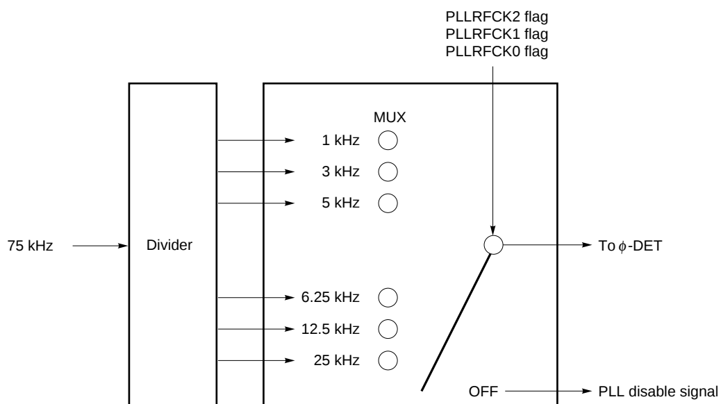
Figure 15-6. Configuration of Reference Frequency Generator
