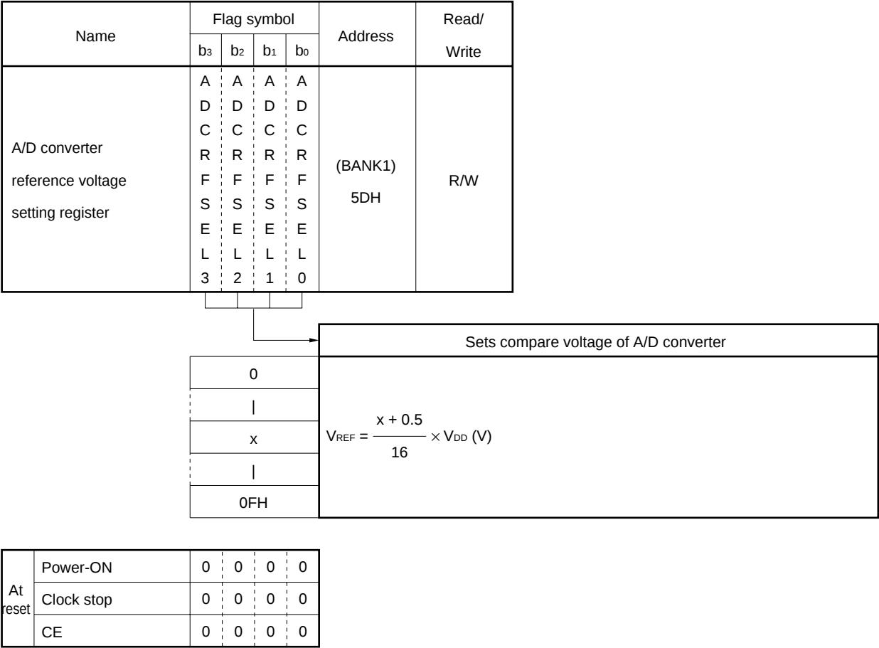
Figure 13-8. Configuration of A/D Converter Reference Voltage Setting Register
