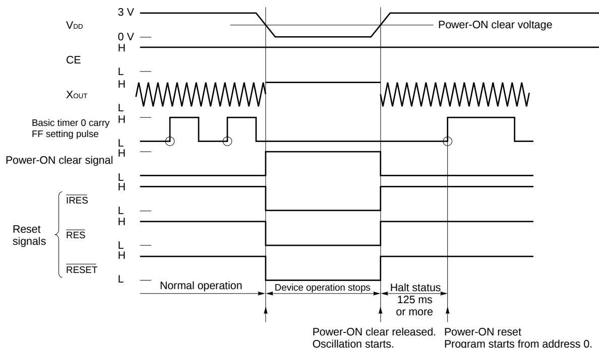
Figure 20-4. Operation of Power-ON Reset
