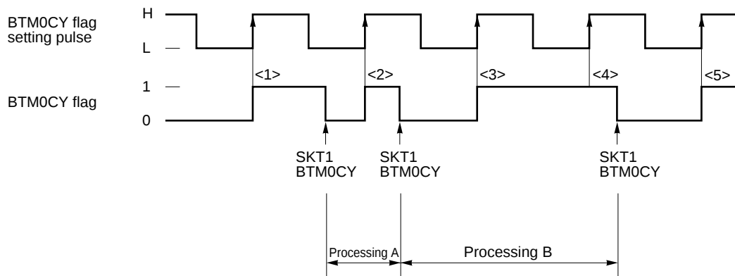
Figure 12-4. Detection of BTM0CY Flag and BTM0CY Flag
