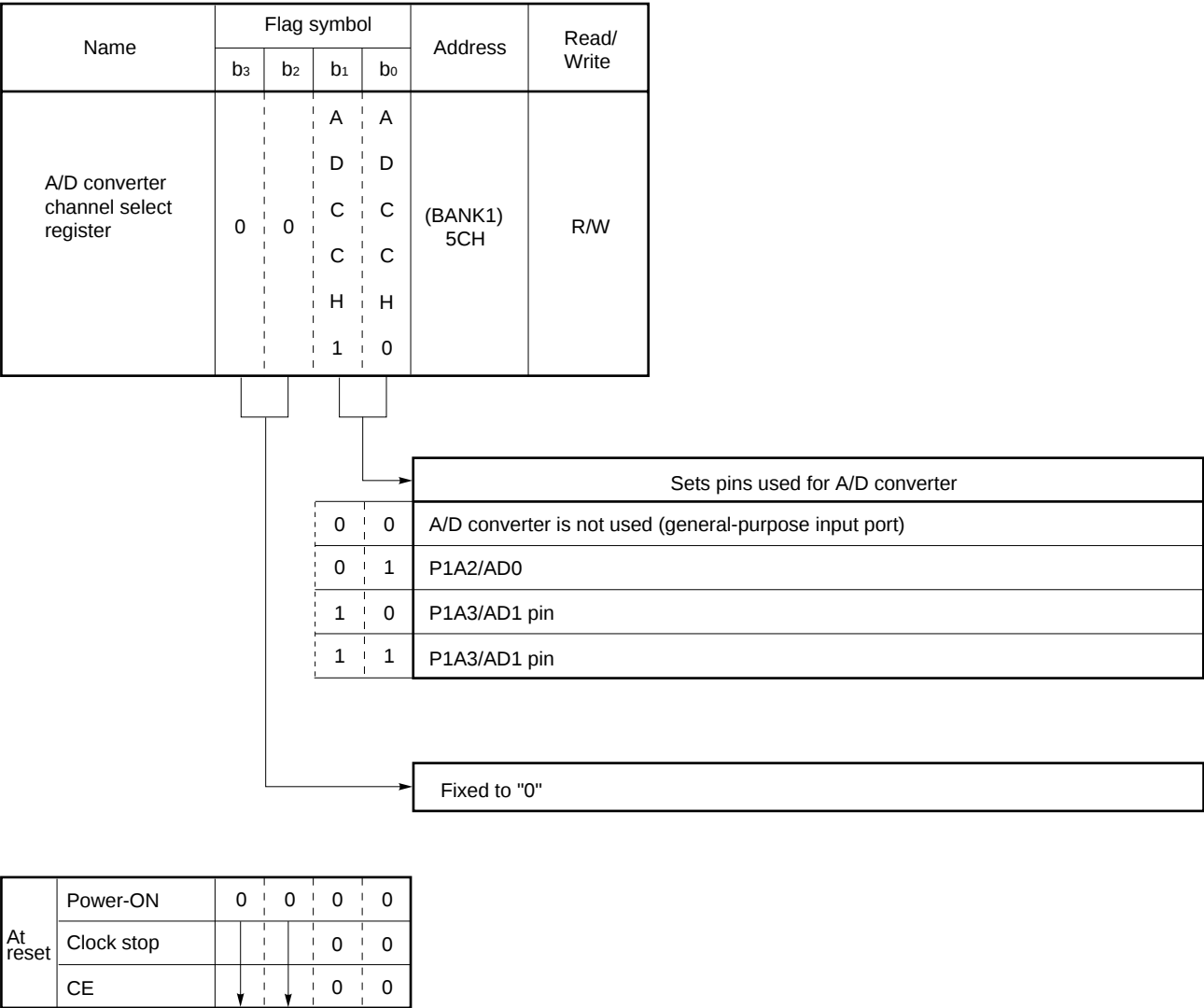
Figure 13-4. Configuration of A/D Converter Channel Select Register
