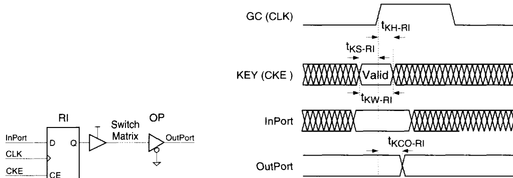
Timing Diagram 9: Key Timing for Register Input, Clock Enable (CKE)
