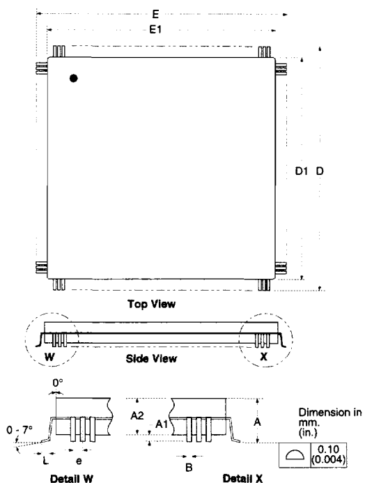
Figure 17: MQAD Package
