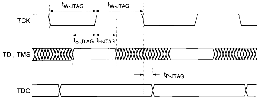
Timing Diagram 16: JTAG Timing
