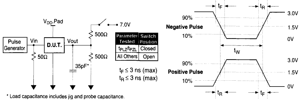
Figure 15: Test Circuit and Waveform Definition
