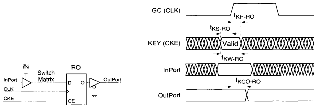
Timing Diagram 10: Key Timing for Register Output, Clock Enable (CKE)
