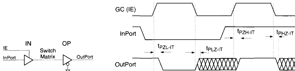
Timing Diagram 6: Input Enable Timing (Flow-through Mode)
