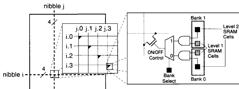
Figure 6: Switch Matrix Control
