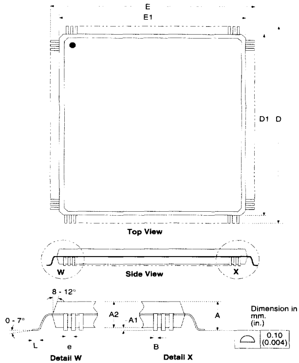
Figure 18: PQFP Package
