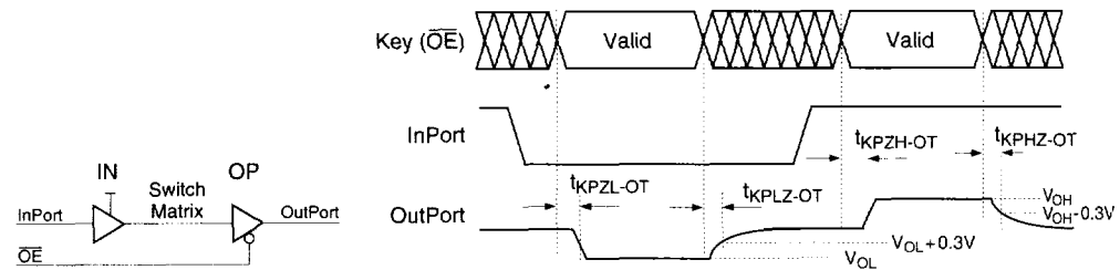
Timing Diagram 11: Key Timing for Output Enable
