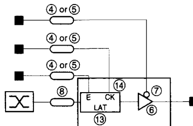
Internal Timing Model 4: Latched Output (From Switch Matrix to Output)
