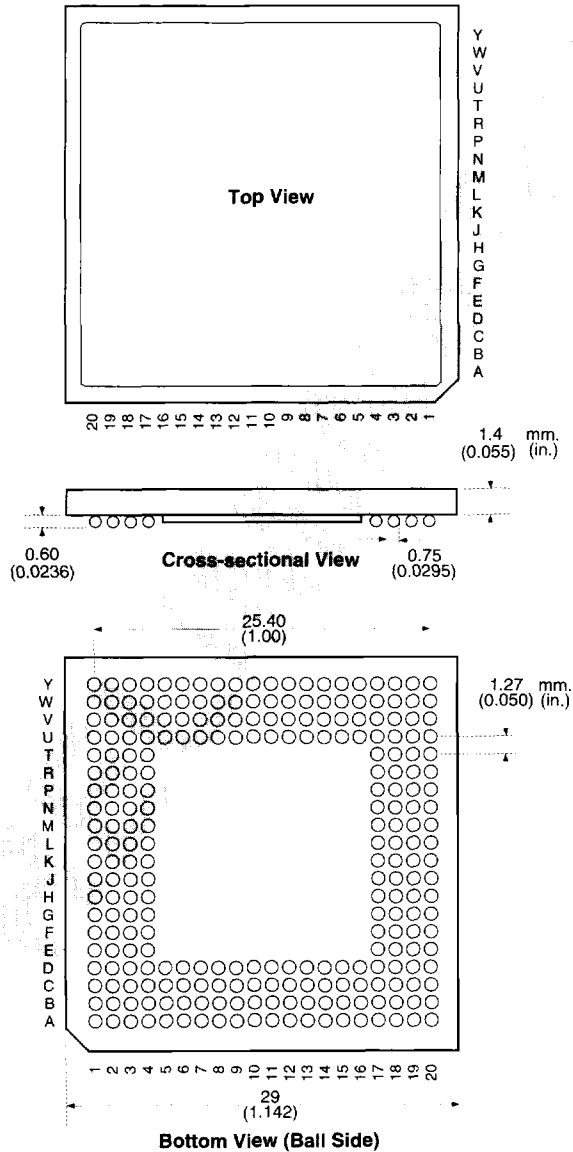
Figure 16: BGA Package Dimensions
