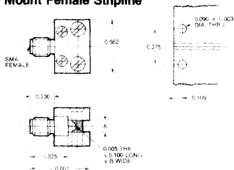
Edge Mount Female Stripline
