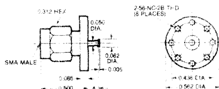
Surface Mount Male Stripline
