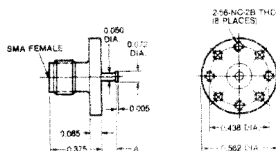
Surface Mount Female Stripline
