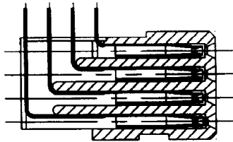
SECTION X-X
