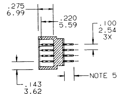
SECTION X-X
