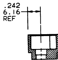
SECTION P-P
