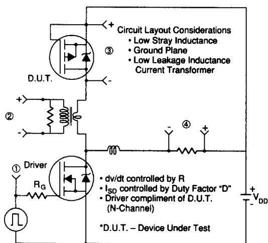
Fig. 13 — Peak Diode Recovery dv/dt Test Circuit
