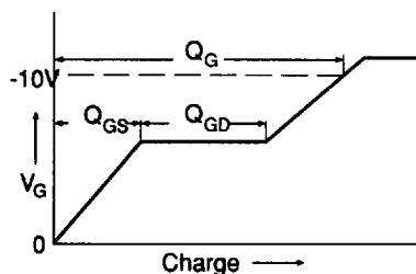
Fig. 14a — Basic Gate Charge Waveform
