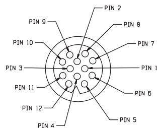
Round (Viking) Cable Models
