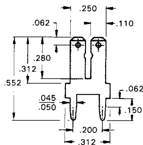
DUAL .110/.250 TAB
