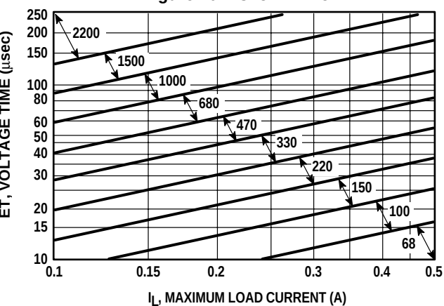
Figure 40. TC2574-ADJ
