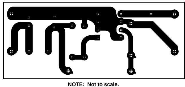
Figure 22. PC Board Layout Copper Side
