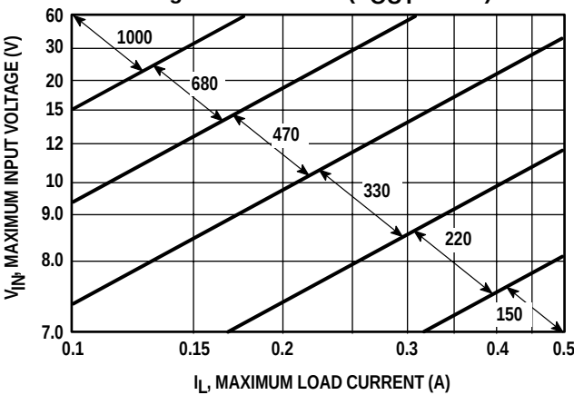
Figure 38. TC2574 ( V_{\text{OUT}} = 5.0\text{V} )
